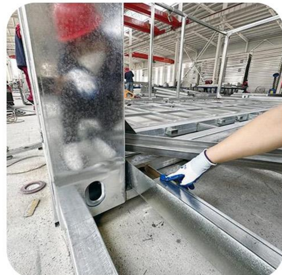
预留框架线路孔 (Reserve holes for frame wiring)
